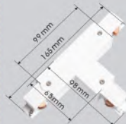
4 wire square T Connector (L) EAN : 69012168 LU-TR4XST-BL White
