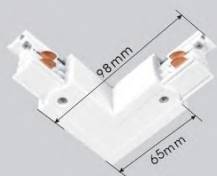
4 wire square L Connector (R) EAN : 69012151 LU-TR4XSL-BR White
